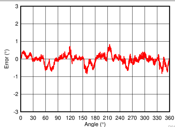
Figure 4-18. Two Sensors Lookup Table Calibrated Error, 26 Cal Points, \approx 2^\circ Peak-to-Peak Error
