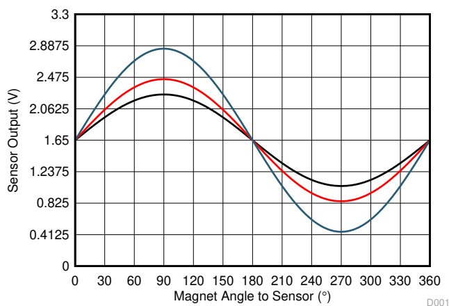
Figure 4-3. One Sensor Uncalibrated Data
