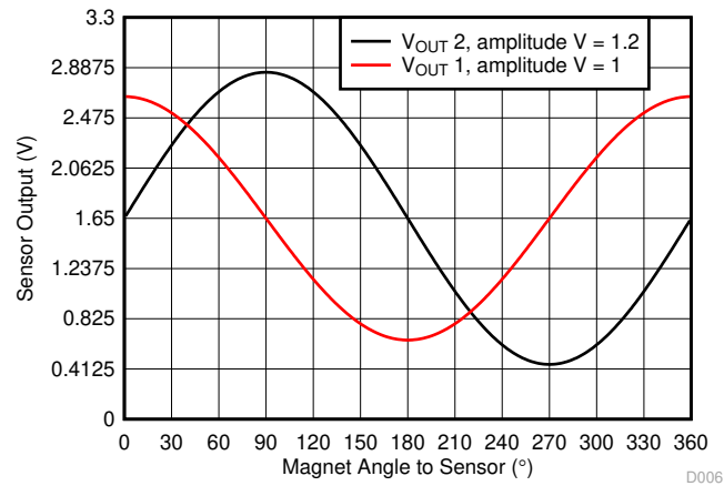
Figure 4-12. Two Sensors Peak Calibrated Data
