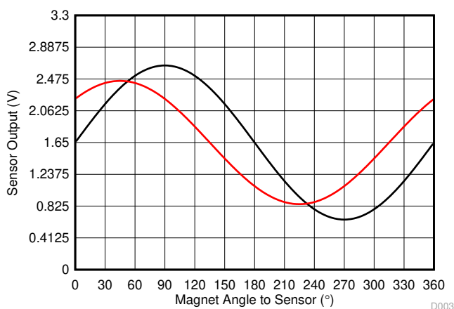
Figure 4-7. Two Sensors 45^\circ Apart Uncalibrated Data
