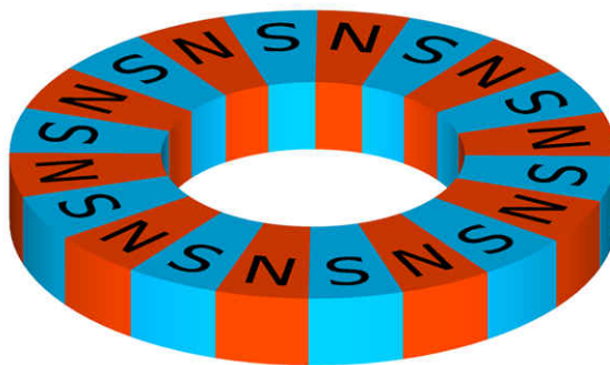
Figure 2-5. Multipole Ring Magnet
