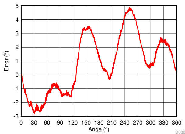
Figure 4-13. Two Sensors Peak Calibrated Error
