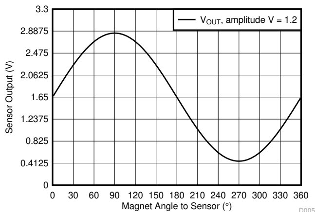
Figure 4-10. One Sensor Peak Calibrated Data
