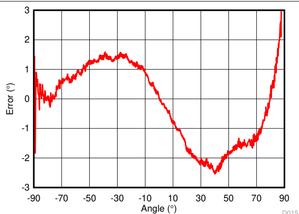
Figure 4-20. One Sensor Peak Calibrated Plus Lookup Table Error, 3 Cal Point, \approx 4^\circ Peak-to-Peak Error
