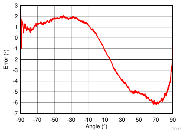
Figure 4-11. One Sensor Peak Calibrated Error
