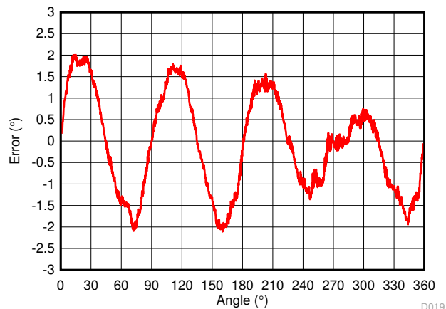
Figure 4-23. Two Sensors Peak Calibrated Plus Lookup Table Error, 8 Cal Points, ≈ 4° Peak-to-Peak Error
