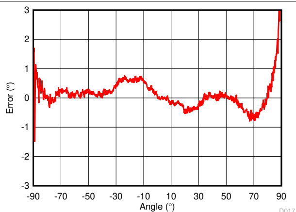
Figure 4-21. One Sensor Peak Calibrated Plus Lookup Table Error, 5 Cal Points, \approx 2^\circ Peak-to-Peak Error
