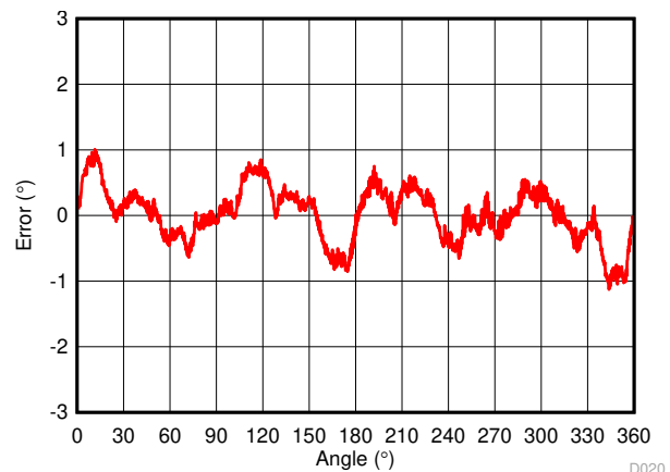
Figure 4-24. Two Sensors Peak Calibrated Plus Lookup Table Error, 14 Cal Points, ≈ 2° Peak-to-Peak Error
