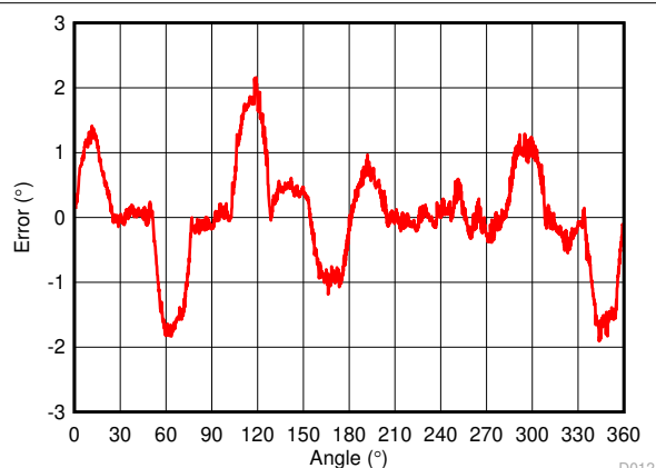
Figure 4-17. Two Sensors Lookup Table Calibrated Error, 14 Cal Points, \approx 4^\circ Peak-to-Peak Error
