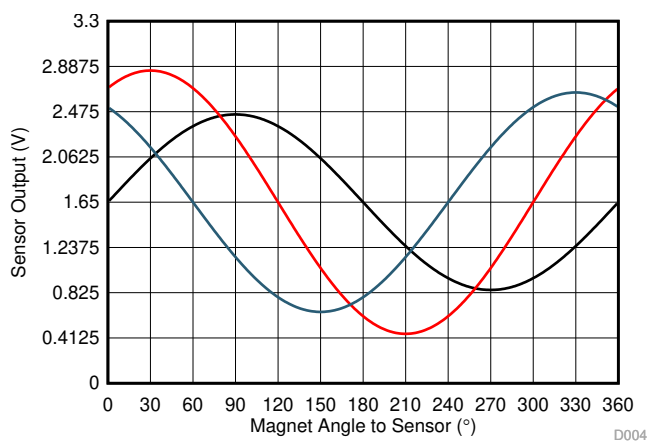
Figure 4-9. Three Sensors 60^\circ Apart Uncalibrated Data
