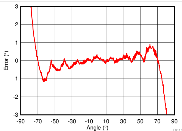
Figure 4-15. One Sensor Lookup Table Calibrated Error, 10 Cal Points, \approx 2^\circ Peak-to-Peak Error
