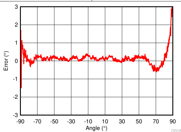
Figure 4-22. One Sensor Peak Calibrated Plus Lookup Table Error, 9 Cal Points, \approx 1^\circ Peak-to-Peak Error
