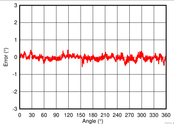
Figure 4-19. Two Sensors Lookup Table Calibrated Error, 45 Cal Points, \approx 1^\circ Peak-to-Peak Error
