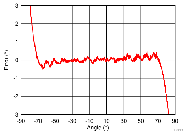
Figure 4-16. One Sensor Lookup Table Calibrated Error, 16 Cal Points, \approx 1^\circ Peak-to-Peak Error
