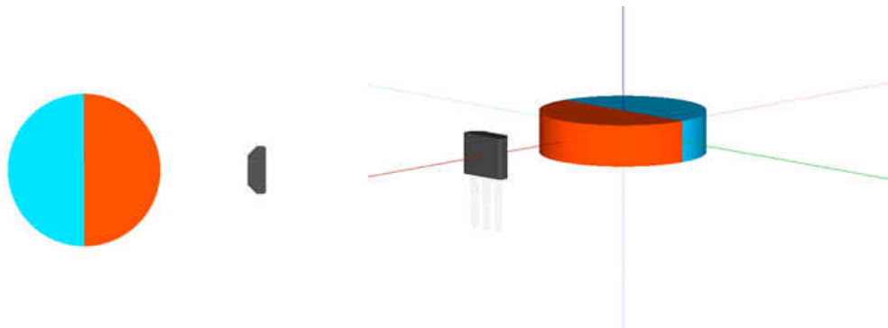
Figure 4-2. One Sensor Near Magnet
