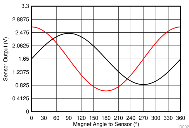
Figure 4-5. Two Sensors 90° Apart Uncalibrated Data
