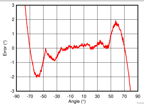
Figure 4-14. One Sensor Lookup Table Calibrated Error, 7 Cal Points, \approx 4^\circ Peak-to-Peak Error
