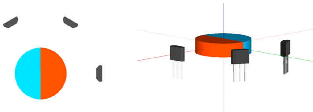
Figure 4-8. Three Sensors 60^\circ Apart
