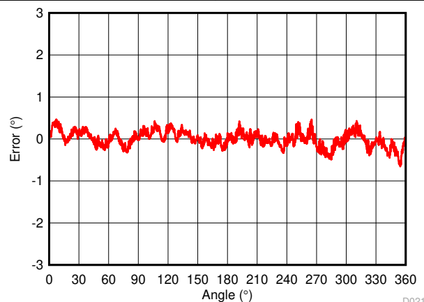
Figure 4-25. Two Sensors Peak Calibrated Plus Lookup Table Error, 25 Cal Points, ≈ 1° Peak-to-Peak Error
