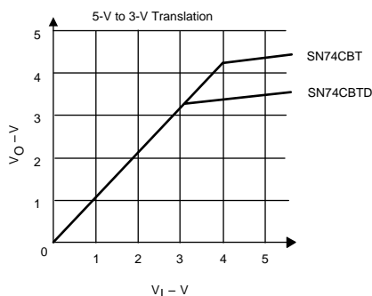
Figure 21. CBT vs CBTD With Internal Diode
